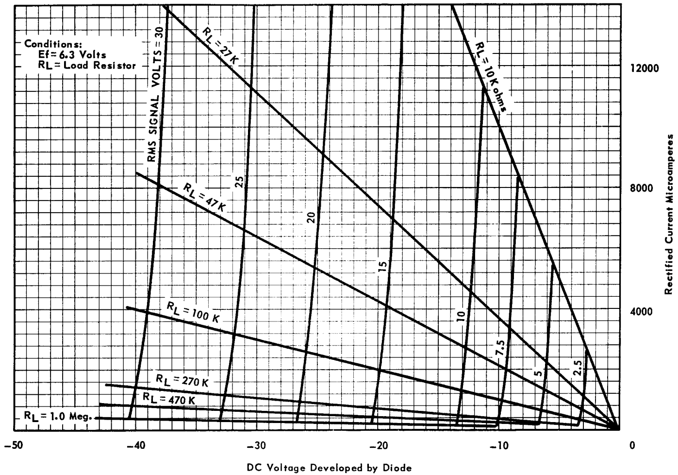
AVERAGE CHARACTERISTICS (Half-Wave Rectification)
